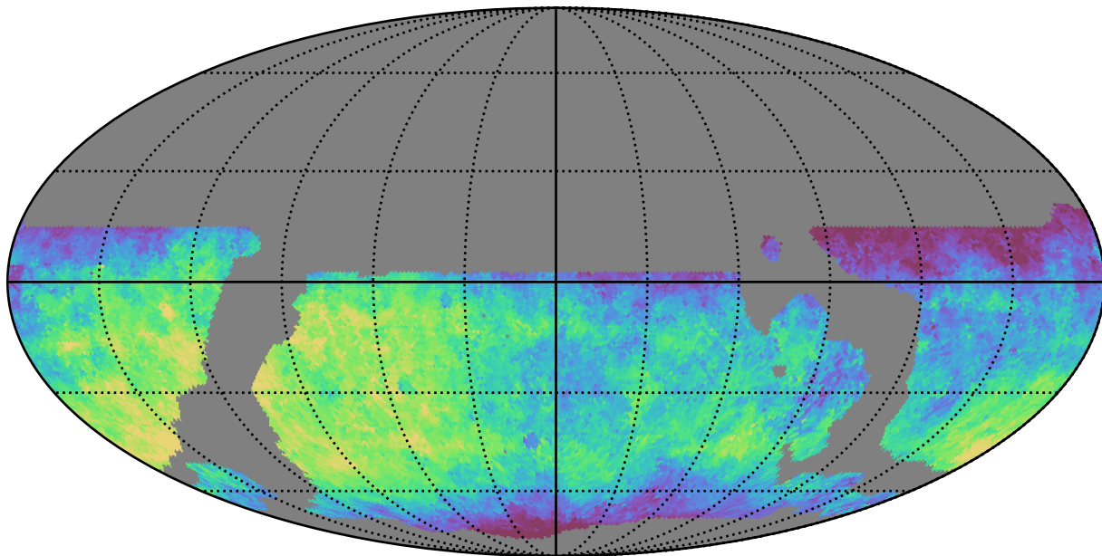
weather_cloudso12v3.4_10yrs WFD y band: Median saturation_mag
