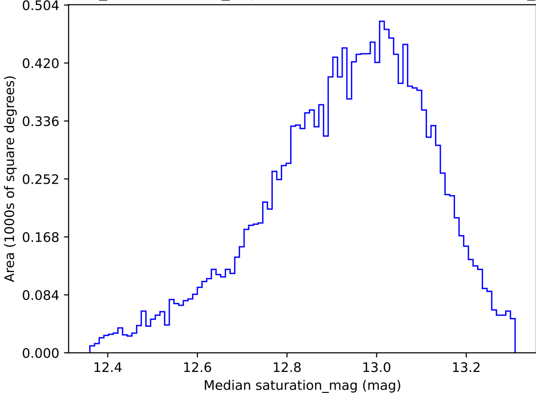
weather_cloudso12v3.4_10yrs WFD u band: Median saturation_mag
