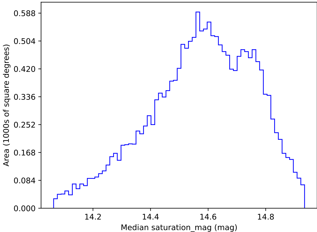
weather_cloudso12v3.4_10yrs WFD r band: Median saturation_mag
