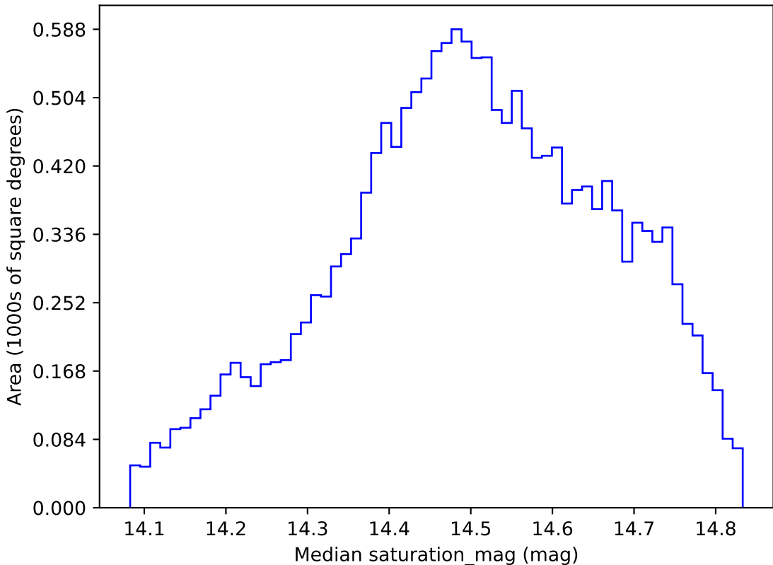
weather_cloudso12v3.4_10yrs WFD i band: Median saturation_mag
