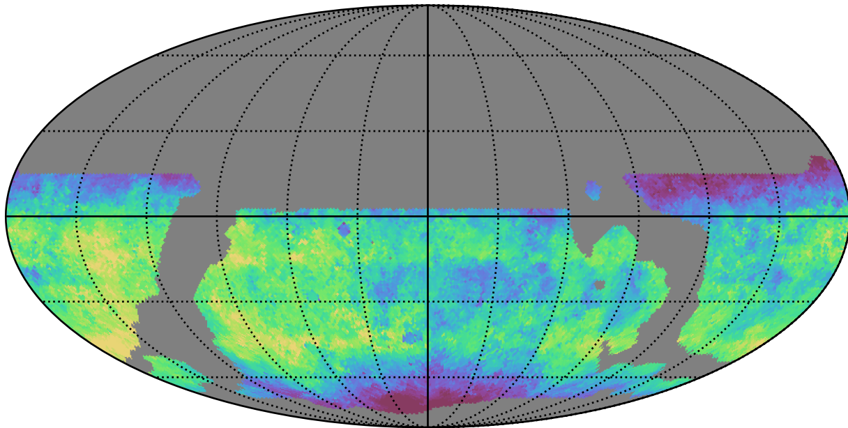
weather_cloudso12v3.4_10yrs WFD g band: Median saturation_mag
