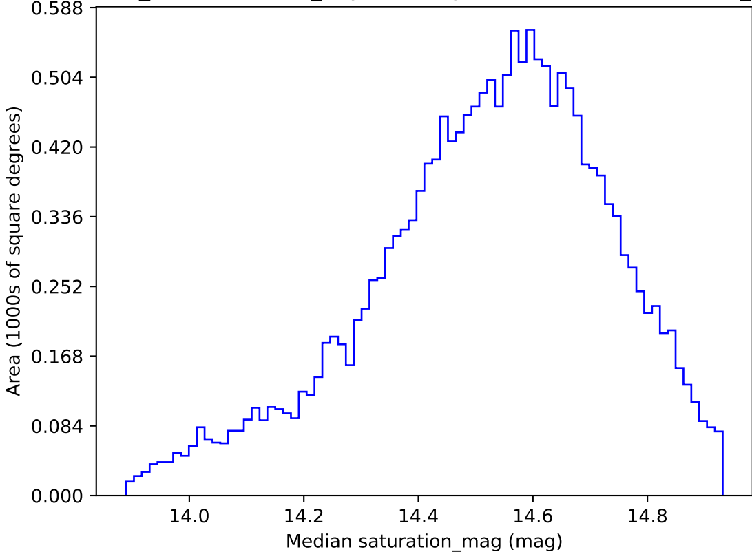
weather_cloudso12v3.4_10yrs WFD g band: Median saturation_mag
