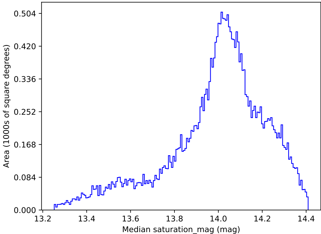
weather_cloudso12v3.4_10yrs All sky z band: Median saturation_mag
