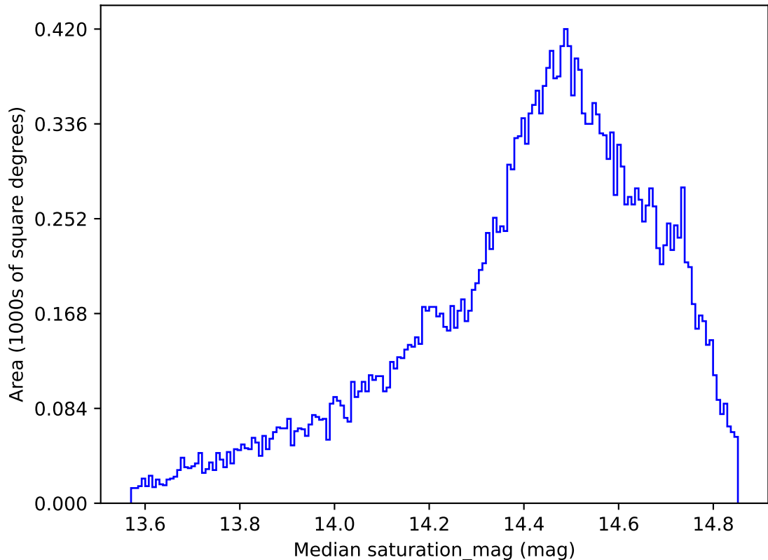
weather_cloudso12v3.4_10yrs All sky i band: Median saturation_mag
