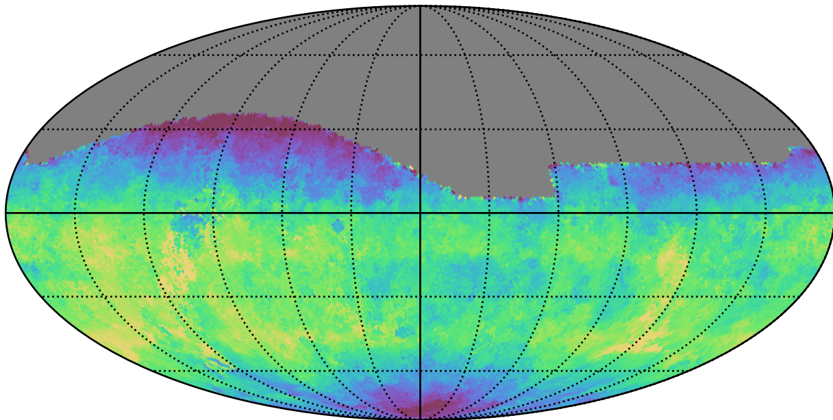
weather_cloudso12v3.4_10yrs All sky g band: Median saturation_mag
