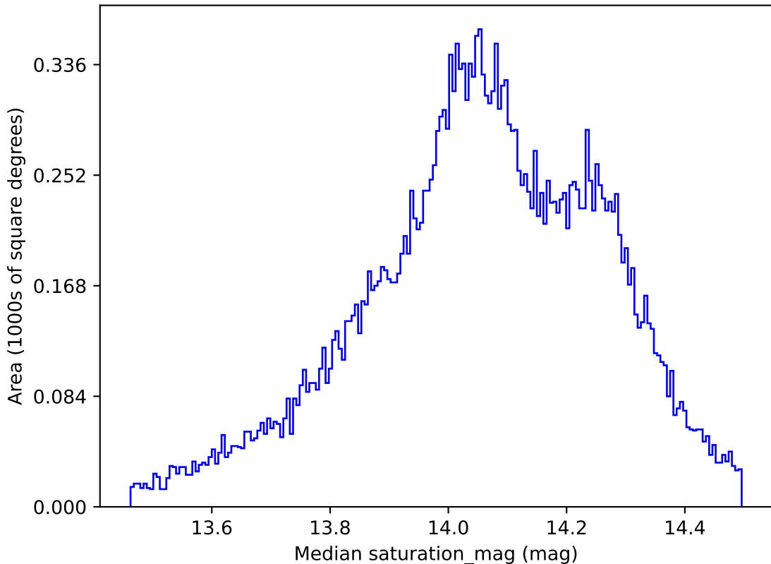
weather_cloudso12v3.4_10yrs All sky all bands: Median saturation_mag
