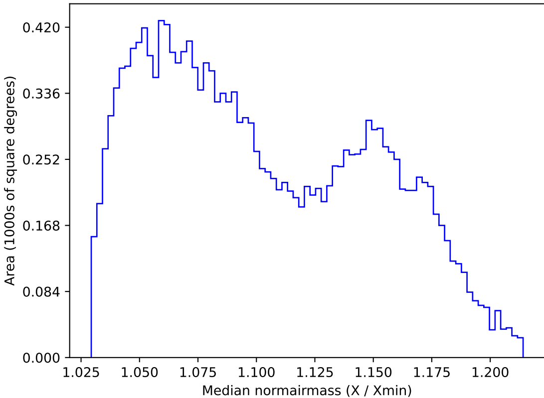
weather_cloudso12v3.4_10yrs WFD z band: Median normairmass
