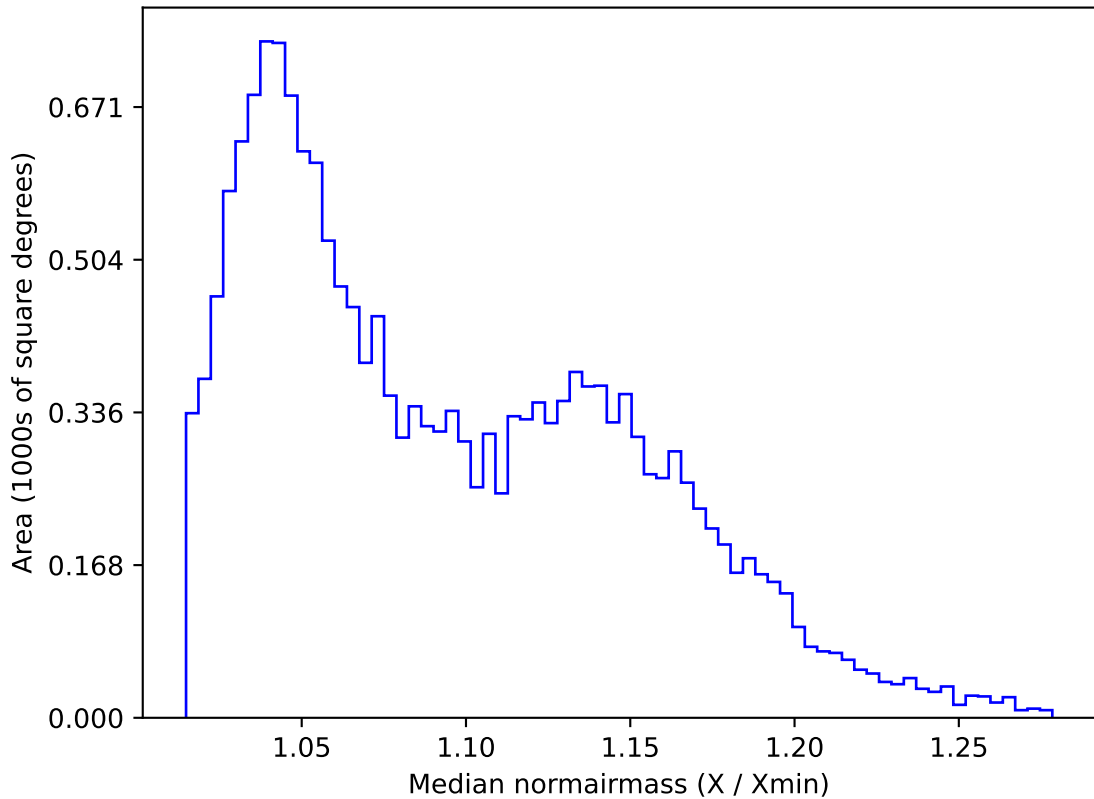
weather_cloudso12v3.4_10yrs WFD u band: Median normairmass
