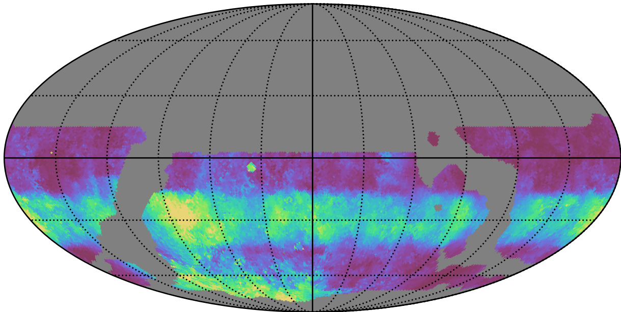
weather_cloudso12v3.4_10yrs WFD g band: Median normairmass
