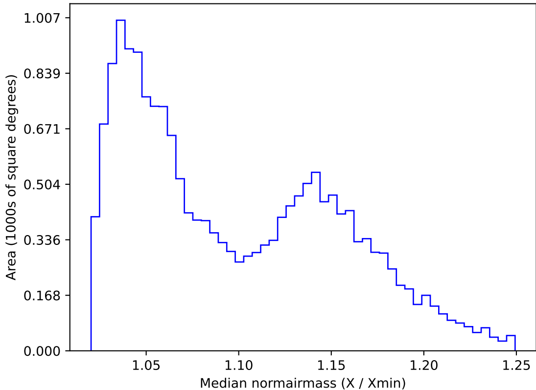
weather_cloudso12v3.4_10yrs WFD g band: Median normairmass
