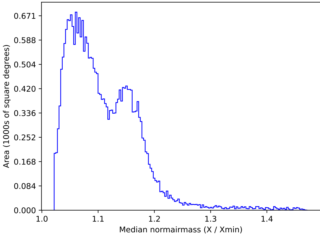
weather_cloudso12v3.4_10yrs All sky z band: Median normairmass
