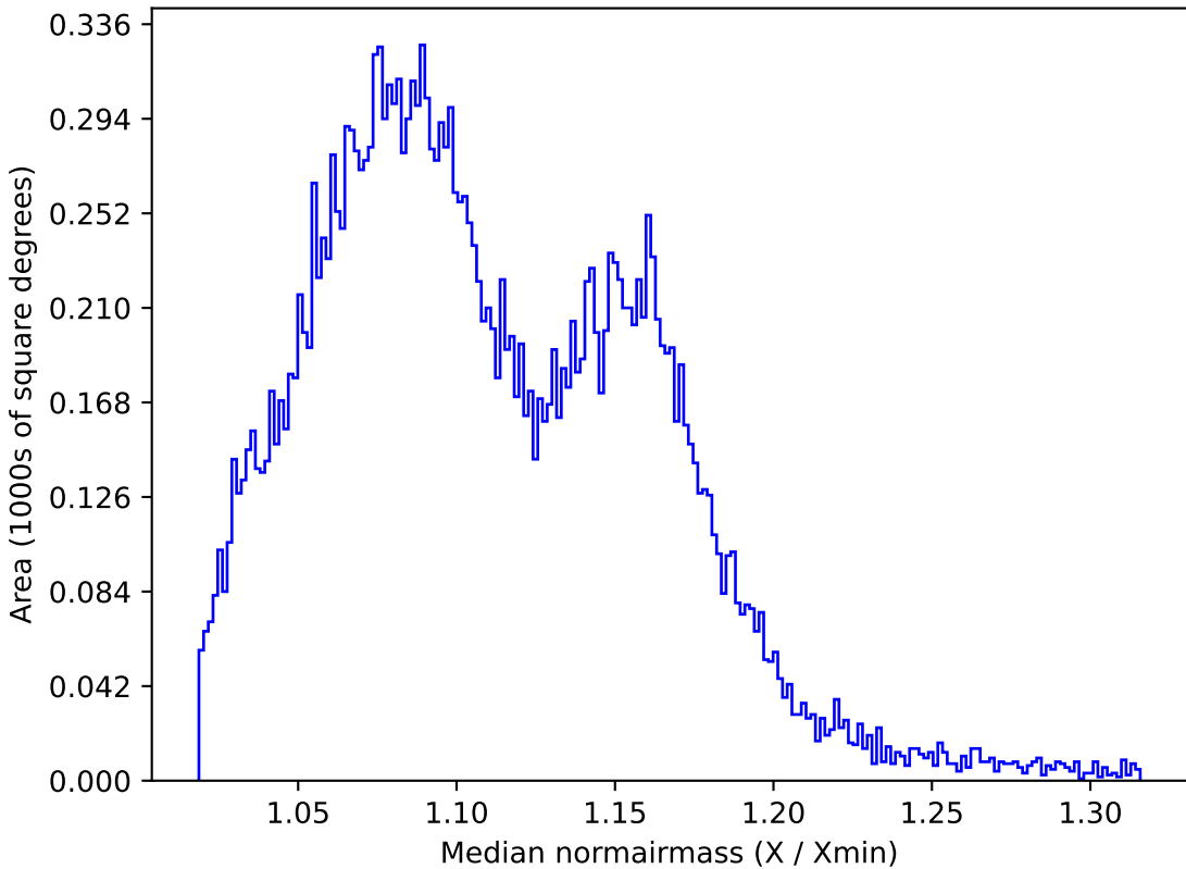
weather_cloudso12v3.4_10yrs All sky y band: Median normairmass
