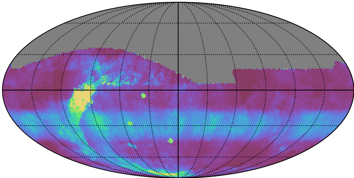
weather_cloudso12v3.4_10yrs All sky r band: Median normairmass
