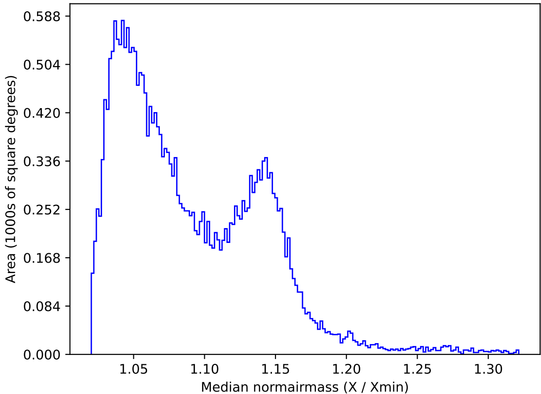
weather_cloudso12v3.4_10yrs All sky i band: Median normairmass
