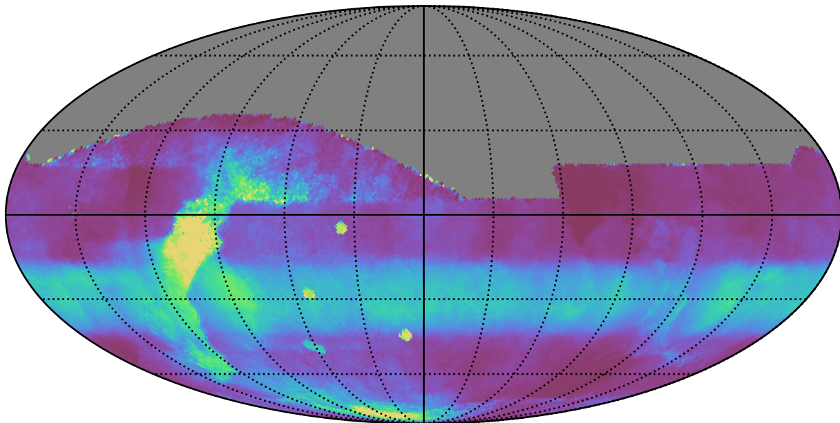
weather_cloudso12v3.4_10yrs All sky all bands: Median normairmass
