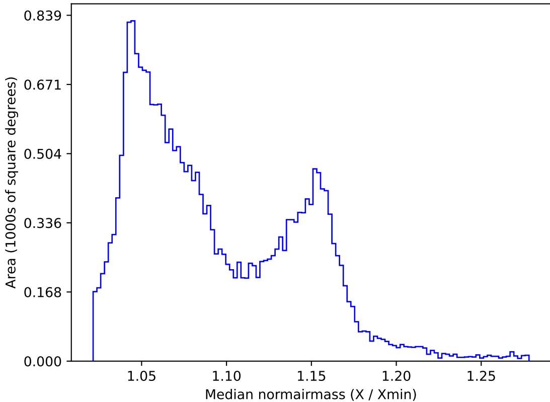
weather_cloudso12v3.4_10yrs All sky all bands: Median normairmass
