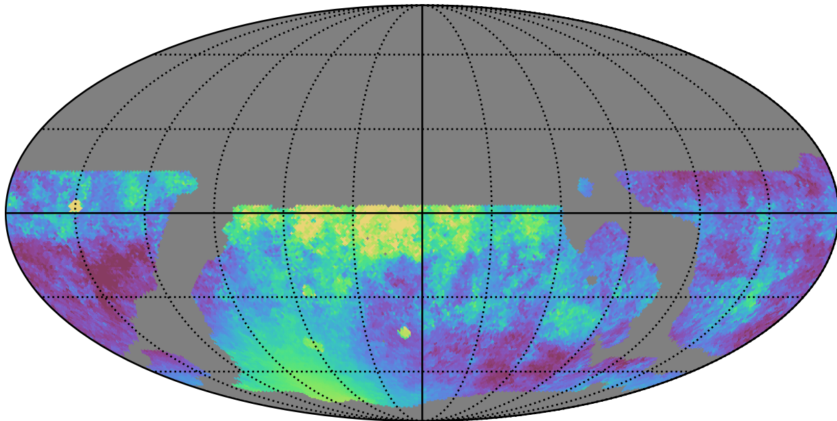
weather_cloudso12v3.4_10yrs WFD z band: Median moonDistance
