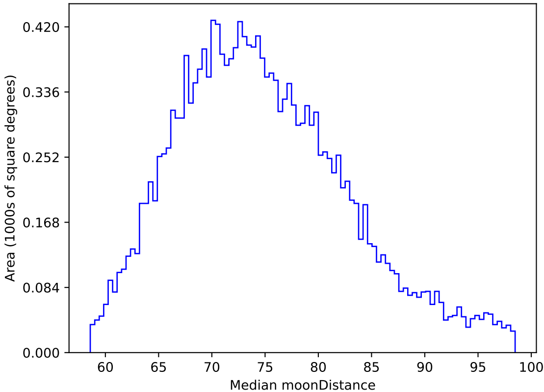
weather_cloudso12v3.4_10yrs WFD z band: Median moonDistance
