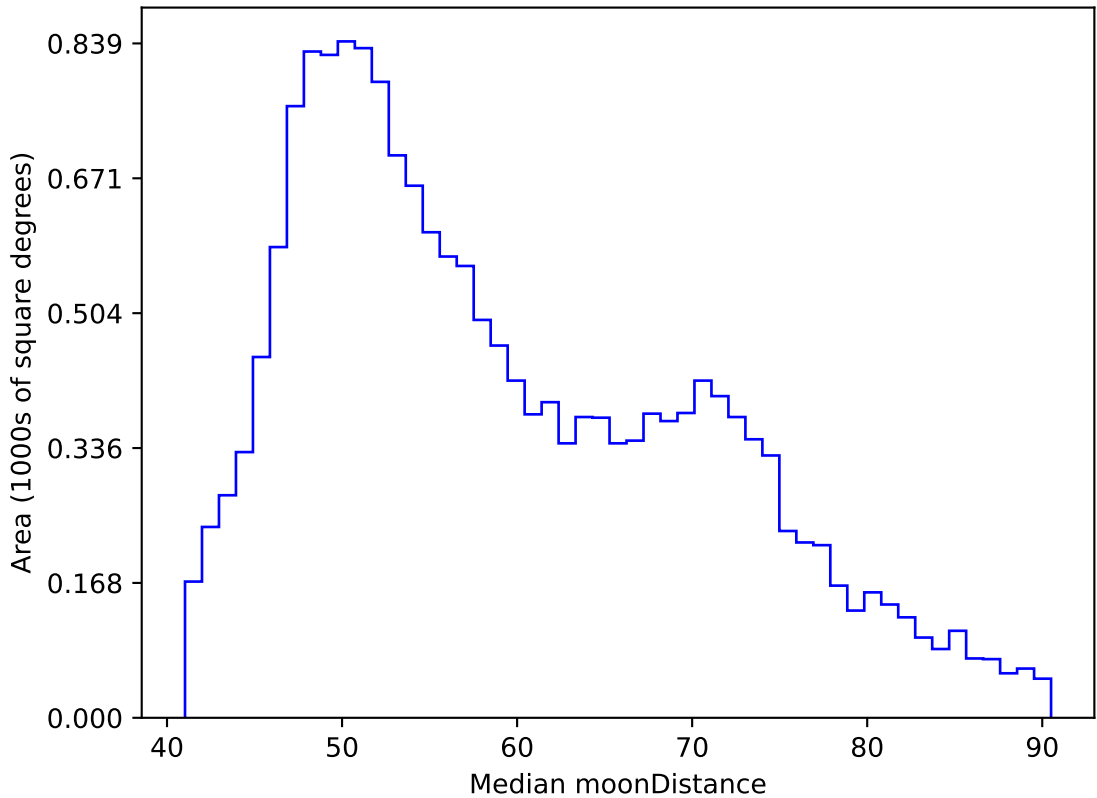
weather_cloudso12v3.4_10yrs WFD y band: Median moonDistance
