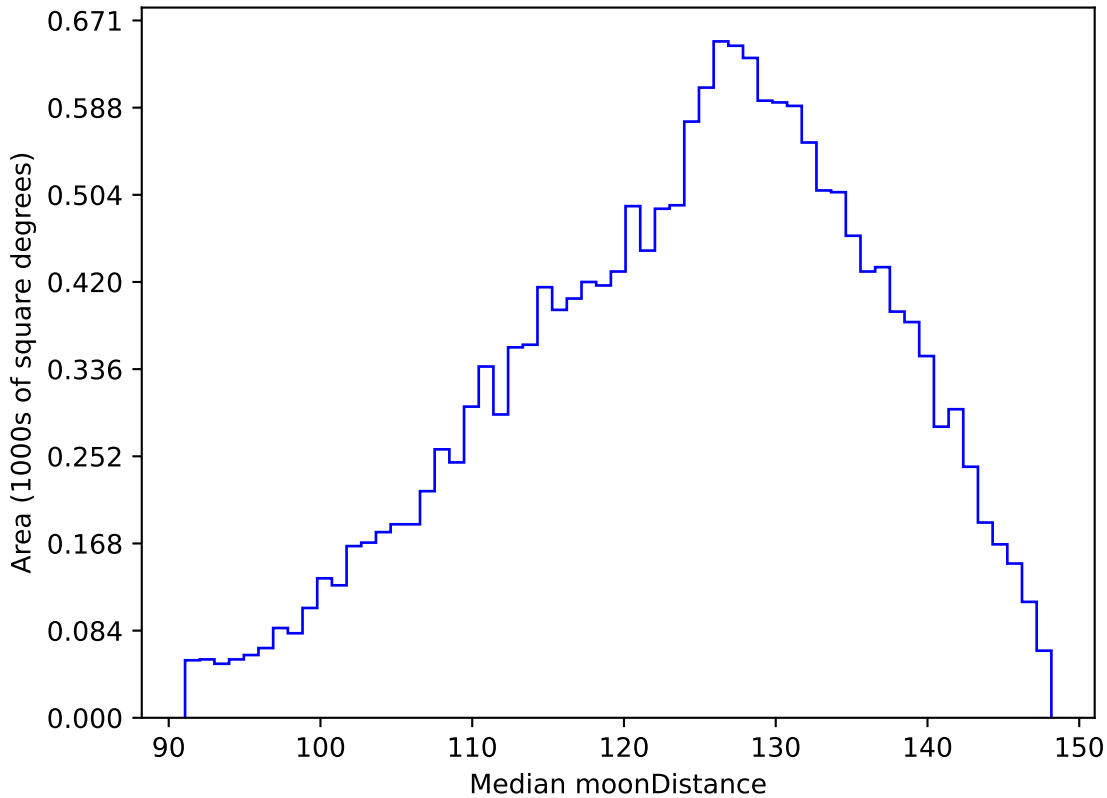
weather_cloudso12v3.4_10yrs WFD u band: Median moonDistance
