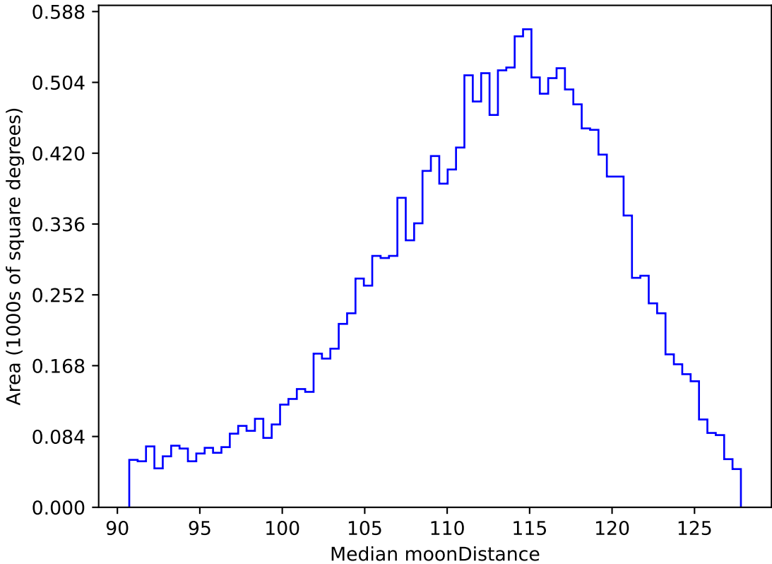
weather_cloudso12v3.4_10yrs WFD r band: Median moonDistance
