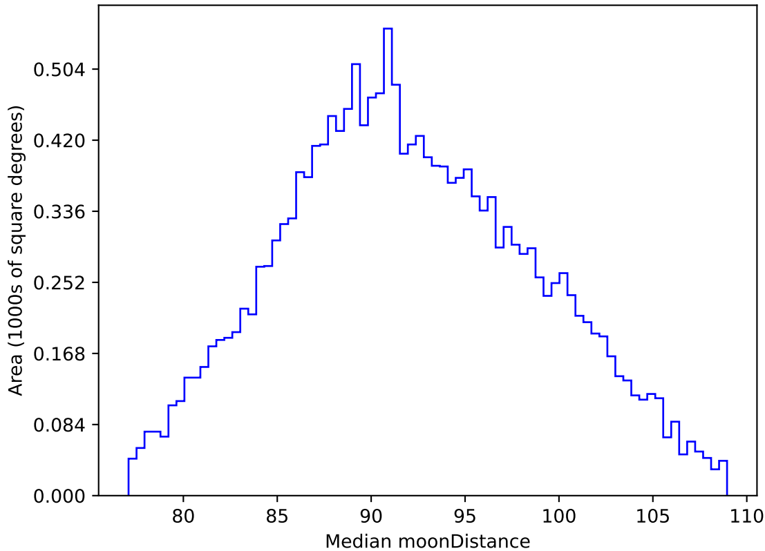
weather_cloudso12v3.4_10yrs WFD i band: Median moonDistance
