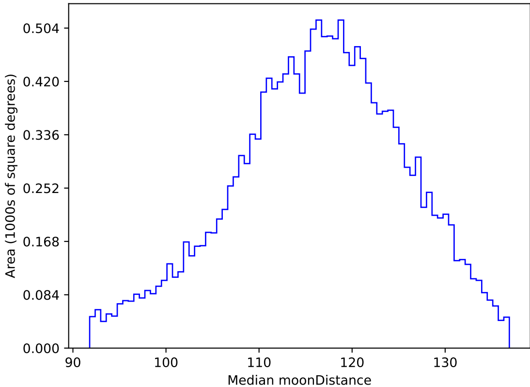
weather_cloudso12v3.4_10yrs WFD g band: Median moonDistance
