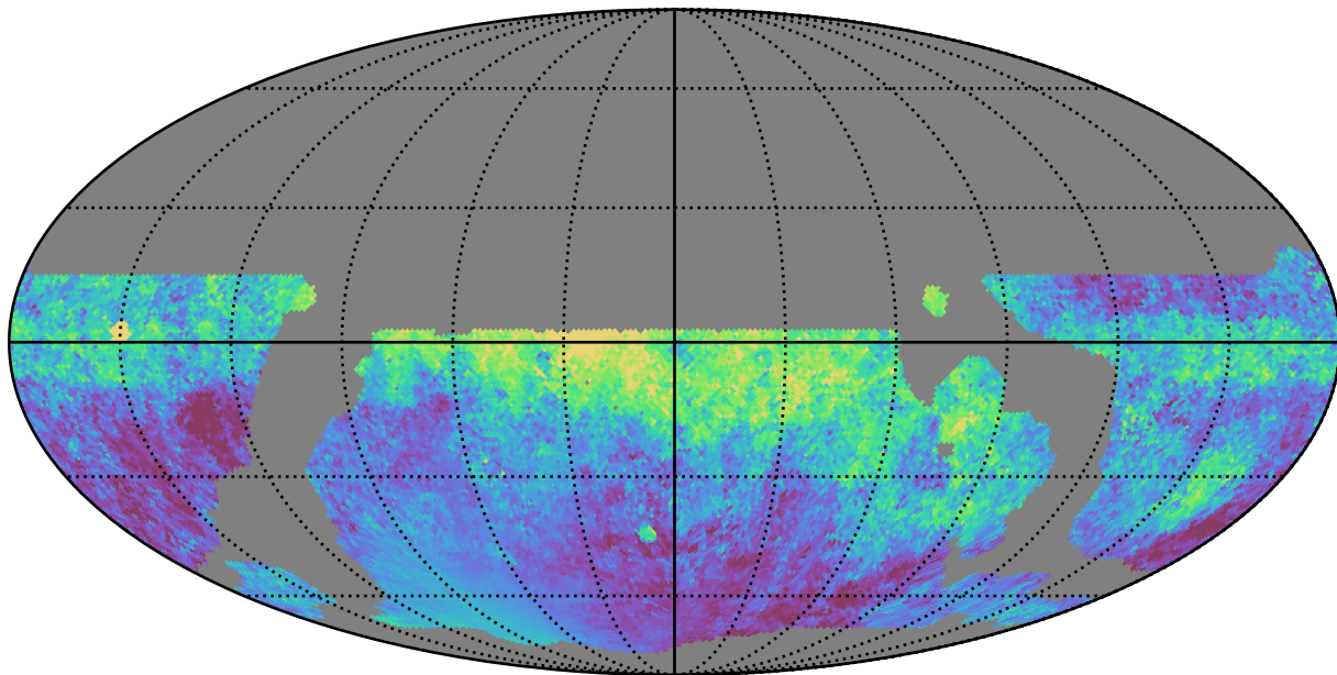
weather_cloudso12v3.4_10yrs WFD all bands: Median moonDistance
