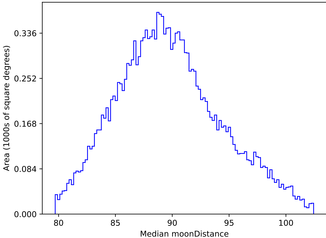
weather_cloudso12v3.4_10yrs WFD all bands: Median moonDistance
