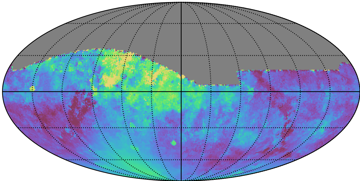
weather_cloudso12v3.4_10yrs All sky z band: Median moonDistance
