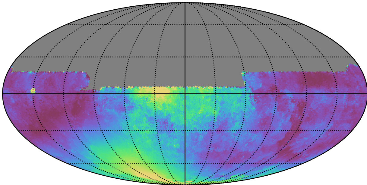
weather_cloudso12v3.4_10yrs All sky y band: Median moonDistance
