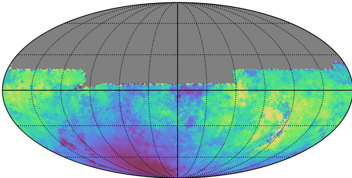
weather_cloudso12v3.4_10yrs All sky u band: Median moonDistance
