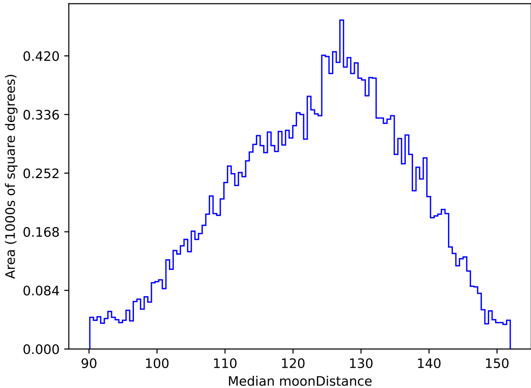
weather_cloudso12v3.4_10yrs All sky u band: Median moonDistance
