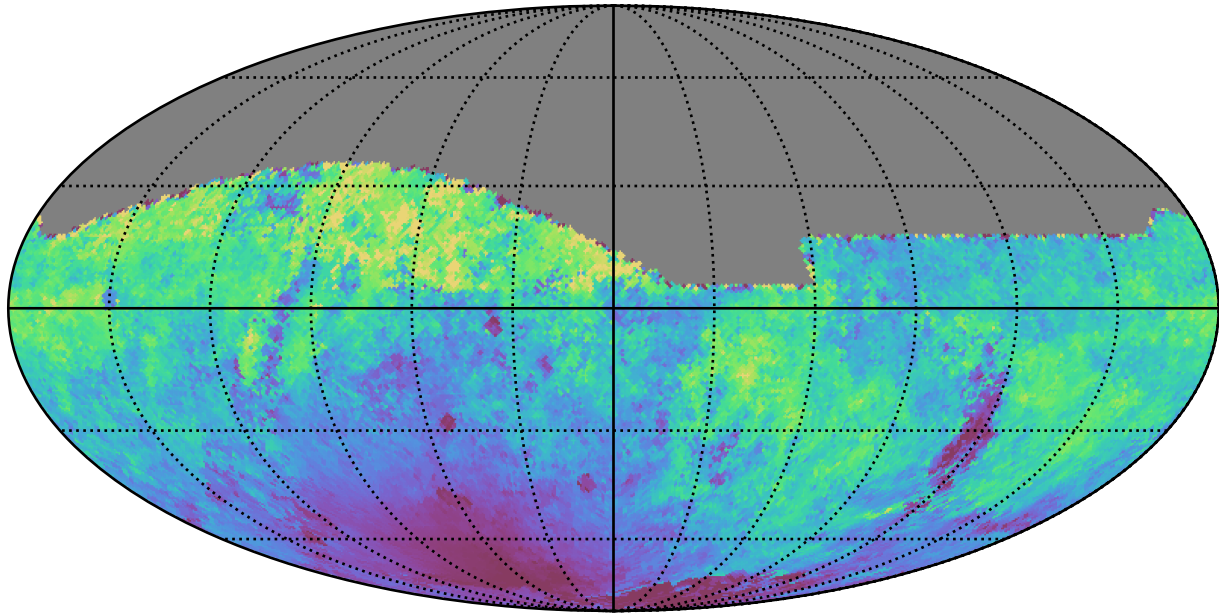
weather_cloudso12v3.4_10yrs All sky r band: Median moonDistance
