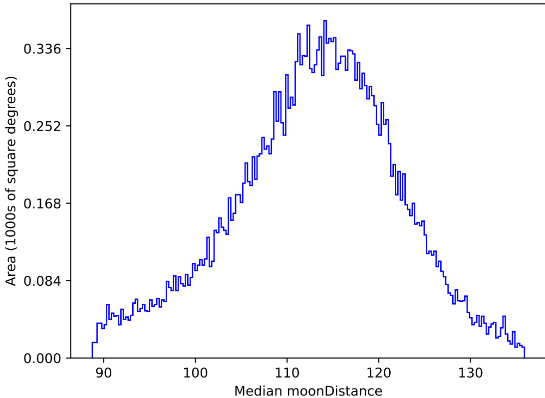
weather_cloudso12v3.4_10yrs All sky r band: Median moonDistance
