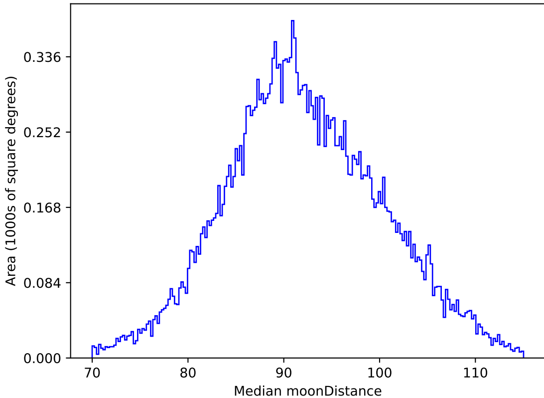
weather_cloudso12v3.4_10yrs All sky i band: Median moonDistance
