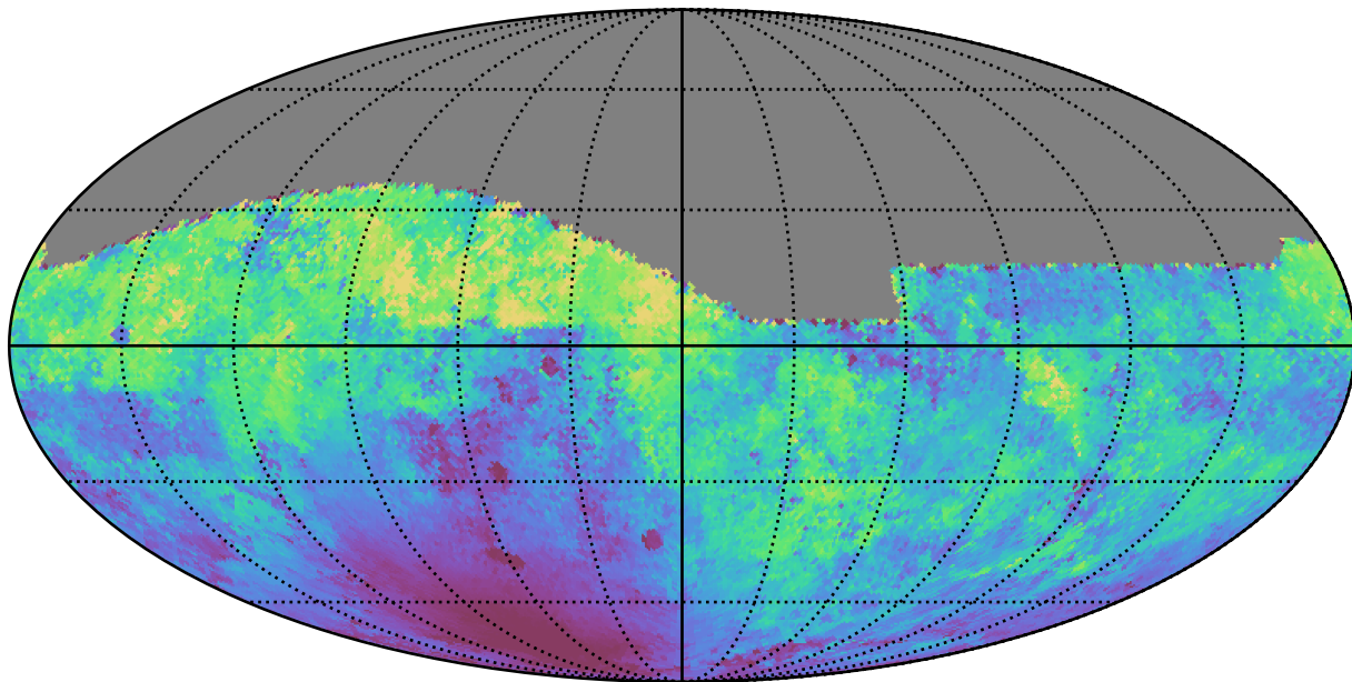
weather_cloudso12v3.4_10yrs All sky g band: Median moonDistance
