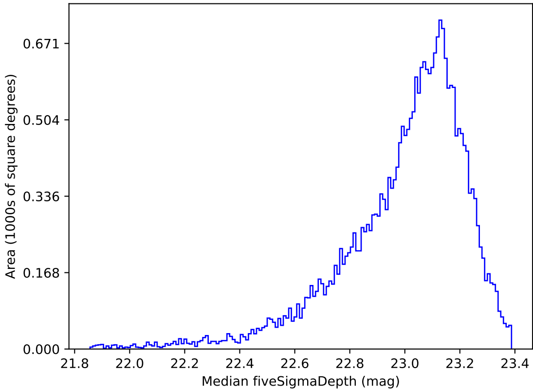
weather_cloudso12v3.4_10yrs Yr 1 z band: Median fiveSigmaDepth
