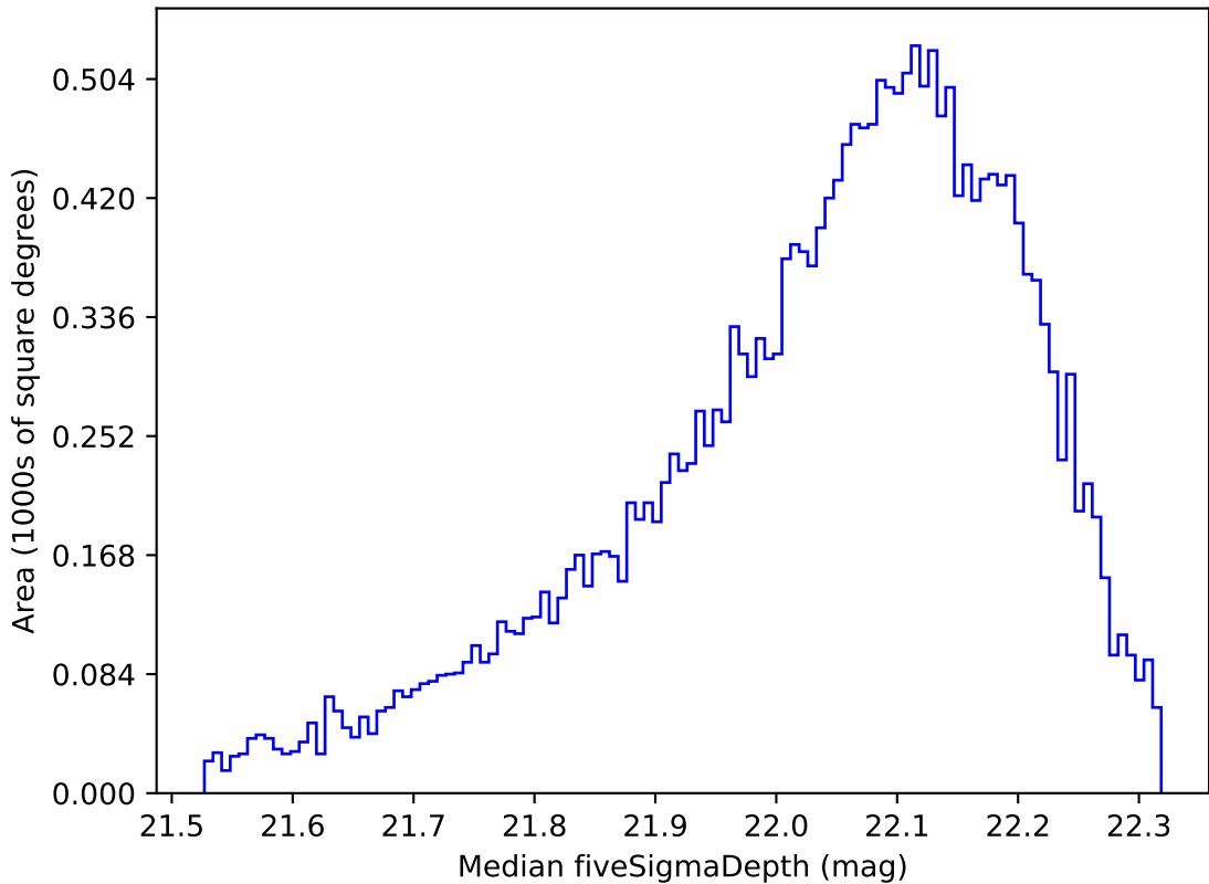
weather_cloudso12v3.4_10yrs Yr 1 y band: Median fiveSigmaDepth
