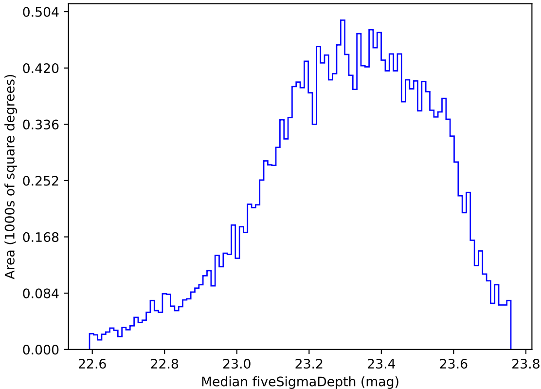
weather_cloudso12v3.4_10yrs Yr 1 u band: Median fiveSigmaDepth
