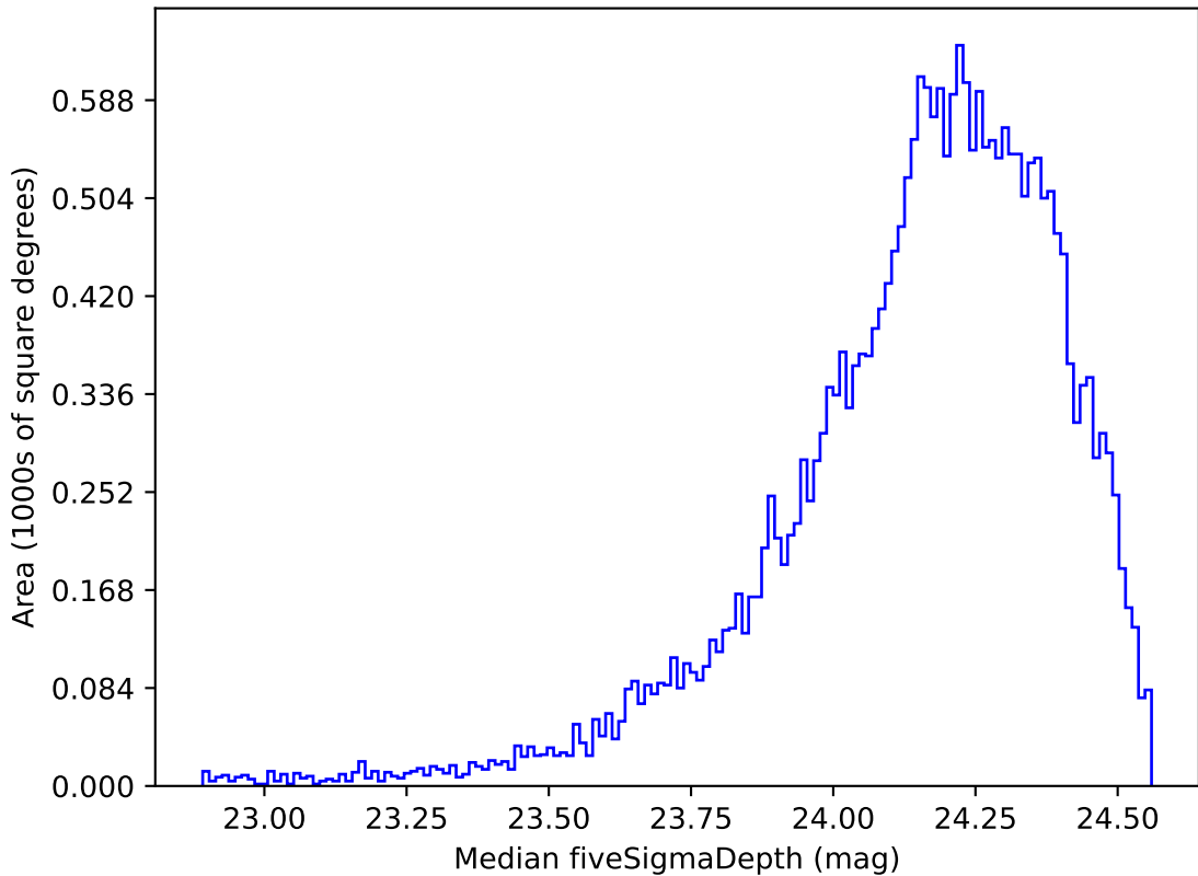
weather_cloudso12v3.4_10yrs Yr 1 r band: Median fiveSigmaDepth
