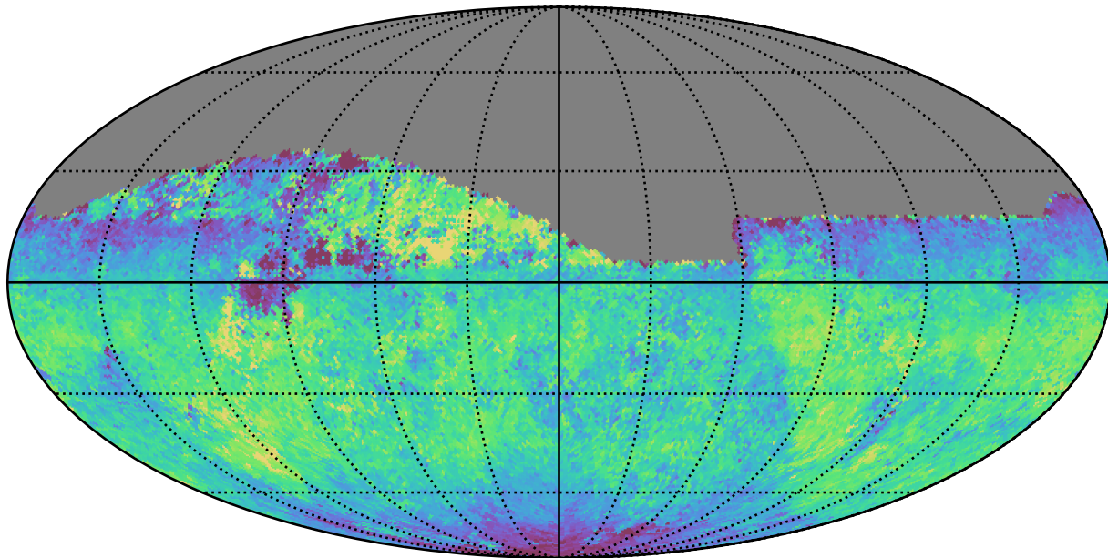
weather_cloudso12v3.4_10yrs Yr 1 all bands: Median fiveSigmaDepth
