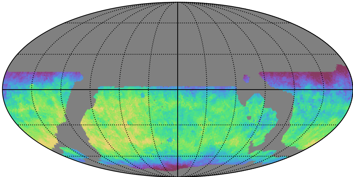
weather_cloudso12v3.4_10yrs WFD y band: Median fiveSigmaDepth
