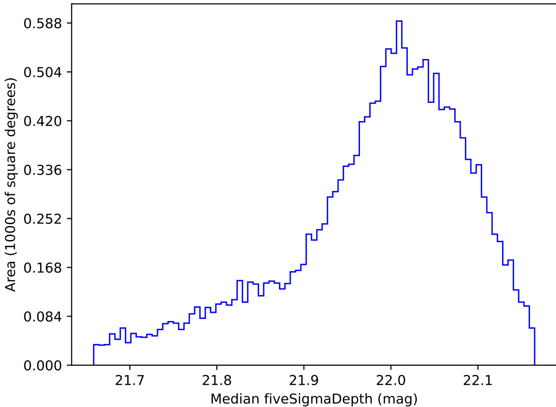
weather_cloudso12v3.4_10yrs WFD y band: Median fiveSigmaDepth
