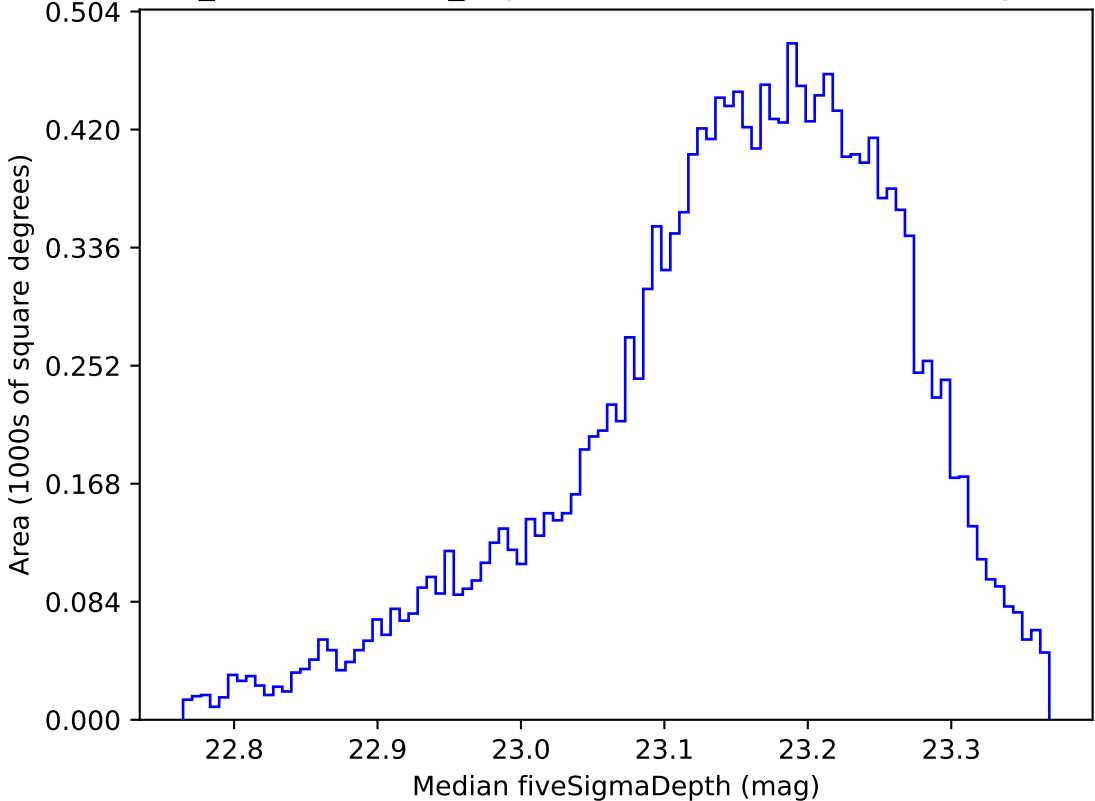
weather_cloudso12v3.4_10yrs WFD u band: Median fiveSigmaDepth
