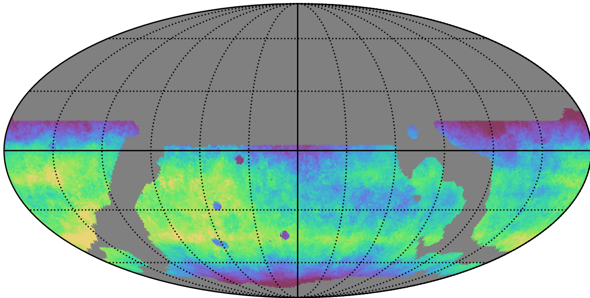
weather_cloudso12v3.4_10yrs WFD r band: Median fiveSigmaDepth
