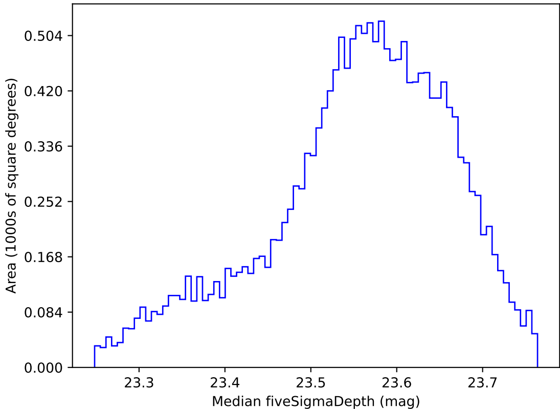
weather_cloudso12v3.4_10yrs WFD i band: Median fiveSigmaDepth
