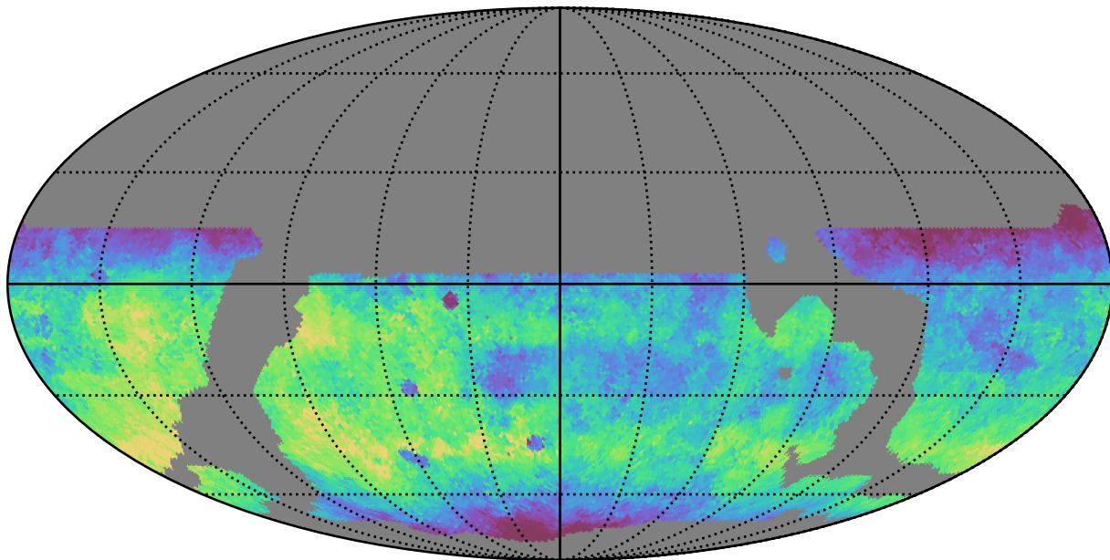
weather_cloudso12v3.4_10yrs WFD g band: Median fiveSigmaDepth
