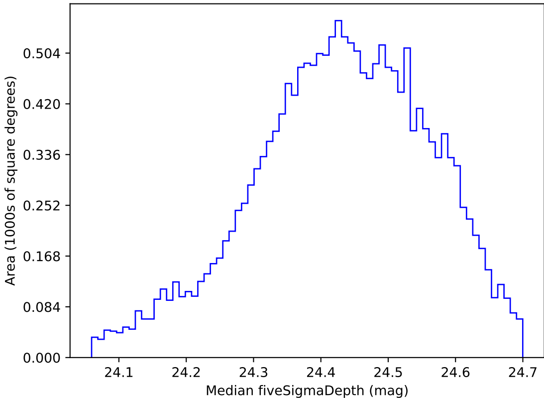
weather_cloudso12v3.4_10yrs WFD g band: Median fiveSigmaDepth
