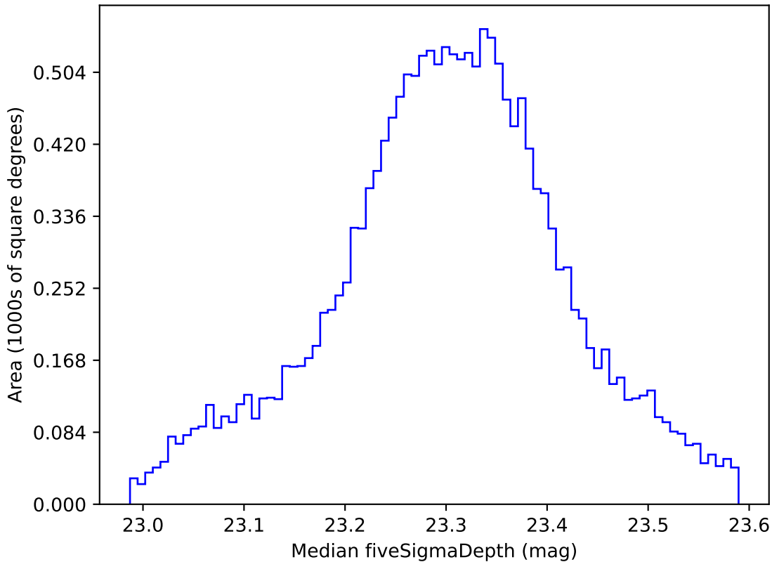
weather_cloudso12v3.4_10yrs WFD all bands: Median fiveSigmaDepth
